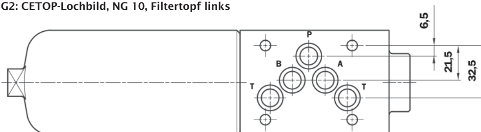
G2: CETOP-Lochbild, NG 10, Filtertopf links
